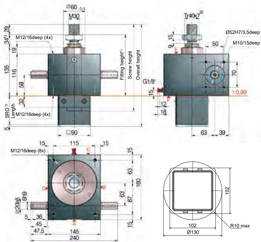
Opening for protective tube square and round
