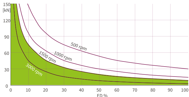
ZE-H 200 Oil lubricated with 8:1 ratio
