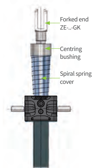
Spiral spring cover attachment for types SN/SL
