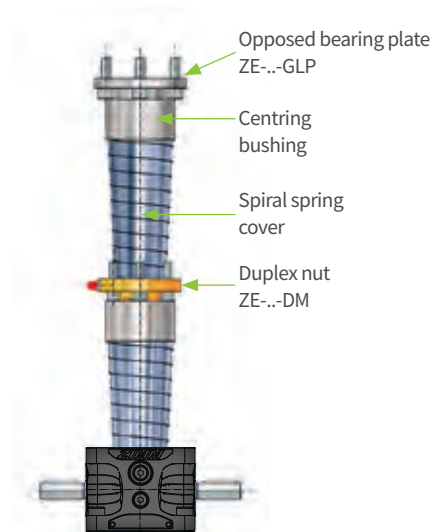
Spiral spring cover attachment for types RN/RL
