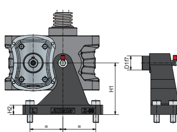
Bearing mount LB (35 - 350)
