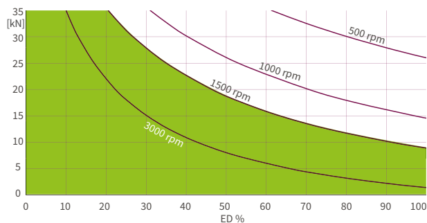
ZE-H 50 Oil lubricated 28:1 ratio
