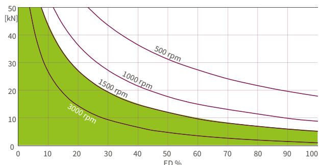
ZE-H 100 Oil lubricated with 9:1 ratio
