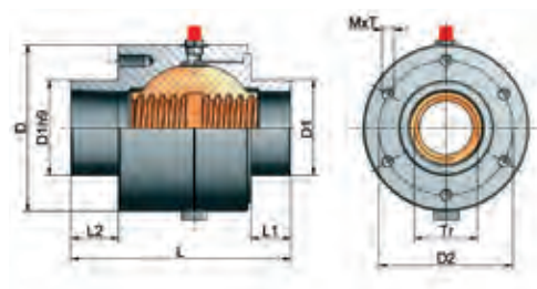
Self-aligning nut PM
