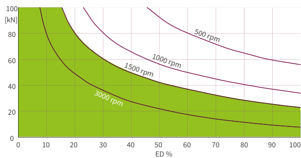
ZE-H 150 Oil lubricated 36:1 ratio
