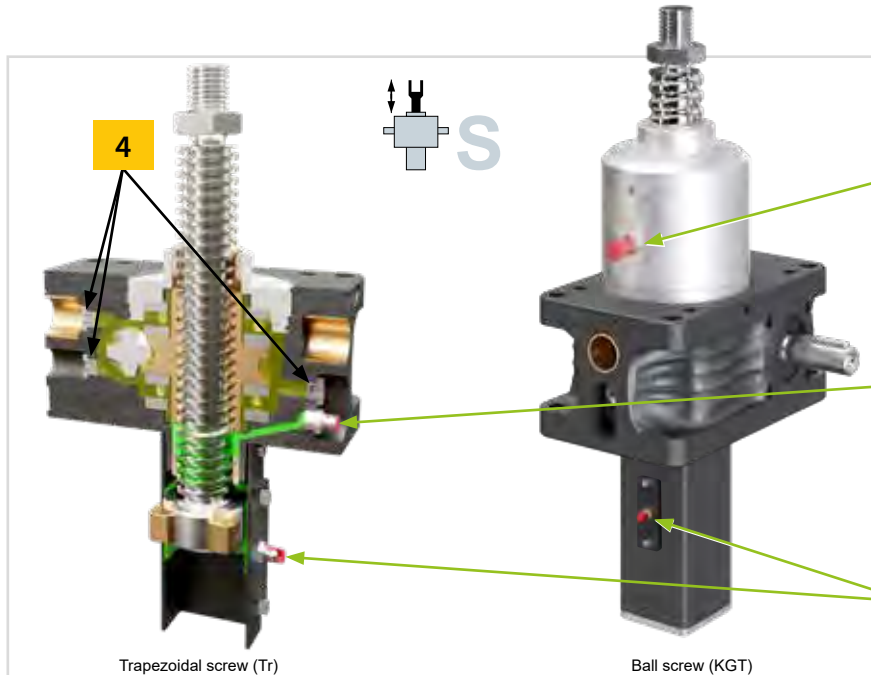
Trapezoidal screw (Tr)
