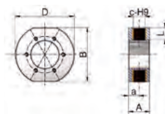
Cardan adapters DMA for duplex nut DM
