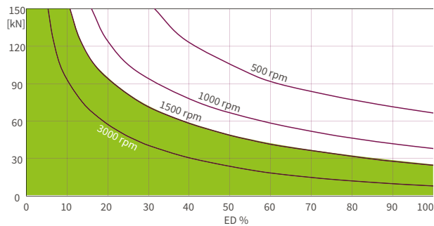
ZE-H 200 Oil lubricated 24:1 ratio
