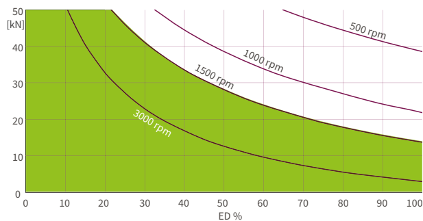
ZE-H 100 Oil lubricated 36:1 ratio
