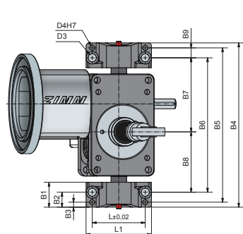
Pivot mounts LB (5 - 25)
